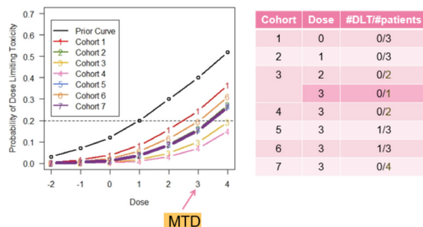
Figure 2 This figure shows the evolution in the estimates of the probabilities of DLTs through successive patient cohorts in the VIOLA Trial which used a continual reassessment method design. The dose-toxicity curves reduced through the first four cohorts as no DLTs were observed before increasing again in cohorts 5 and 6 when DLTs occurred. The MTD was declared at dose level 3 as it had an estimated DLT risk closest to the target toxicity level of 20% (adapted from Craddock et al. 7 ). DLT, dose-limiting toxicity; MTD, maximum tolerated dose.
